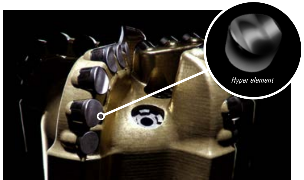
The hyperbolic shape of the Hyper element mitigates the severe bit balling that commonly occurs with flat PDC cutters by creating small cuttings chips, improving cuttings removal and increasing ROP.
