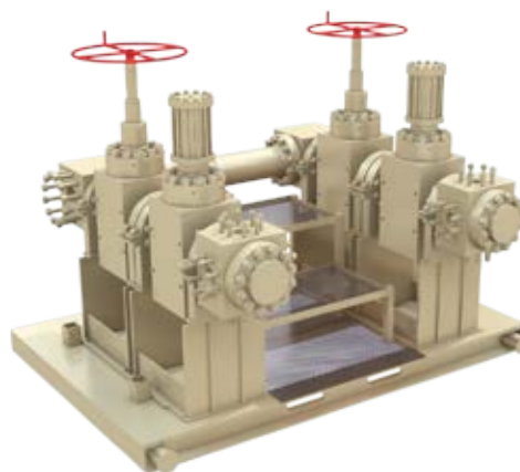
Two-leg manual valve and hydraulic valve isolation frac manifold
