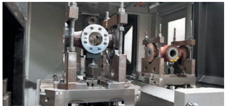
Valve cavities going through finish machining process
