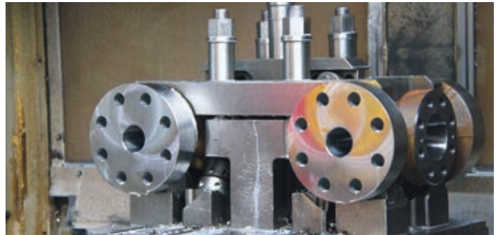
Valve bodies in fixture for machining
