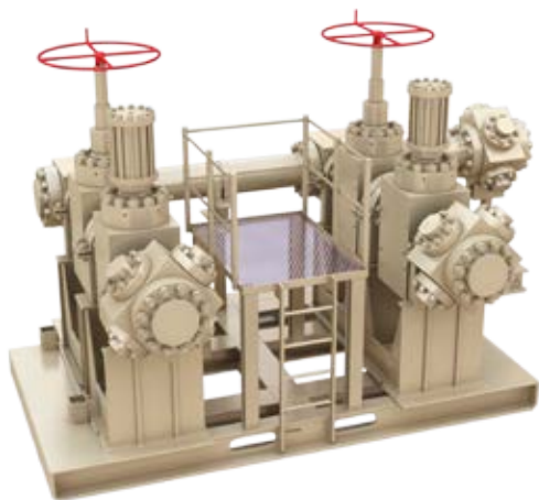
Two-leg manual valve and hydraulic valve isolation frac manifold with safety platform for safe access to valves
