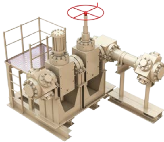
One-leg frac manifold with safety platform for safe access to valves
