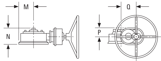
DYNATORQUE accessories gearbox. Stem size: 5 in, 7.5 in, and 9 in.
