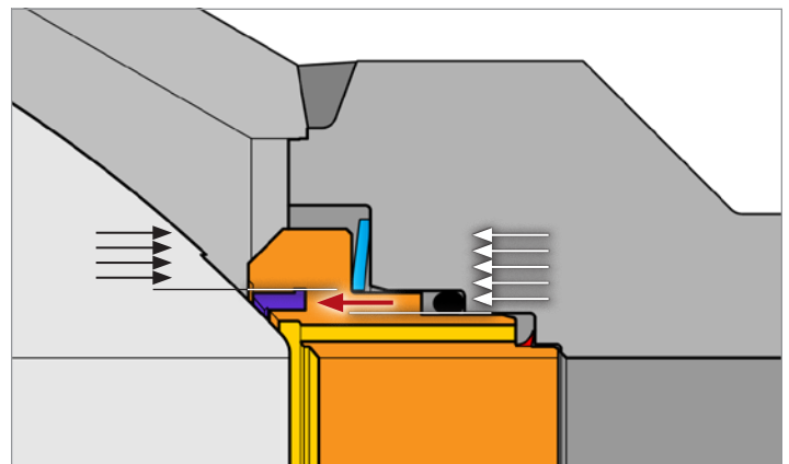
Downstream sealing.
