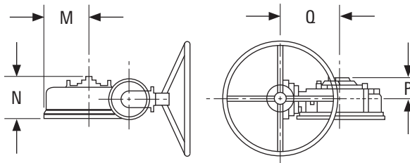
DYNATORQUE accessories gearbox. Stem size: 3 in and 4 in.
