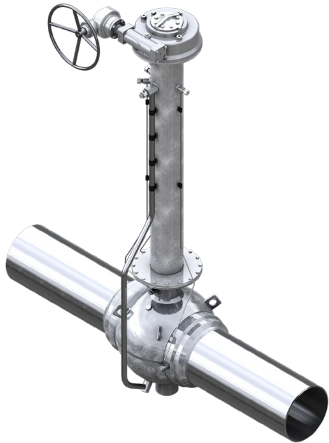
Stem extension and transition pieces for remote operation.
