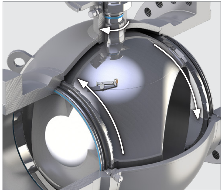
Rotating seat rings.
