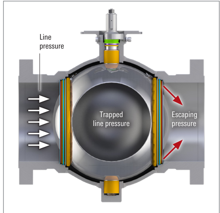
Automatic internal relief of body pressure.
