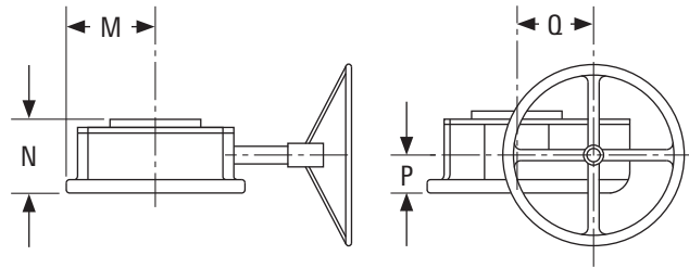
DYNATORQUE accessories gearbox. Stem size 1 in, 1.5 in, 2 in, and 3 in.
