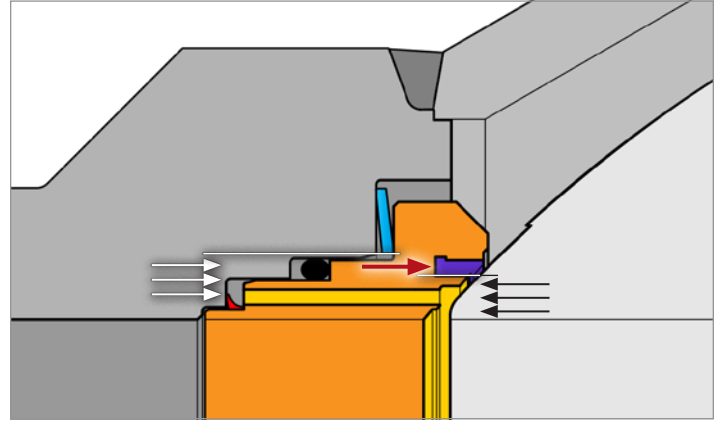
Conventional upstream sealing.
